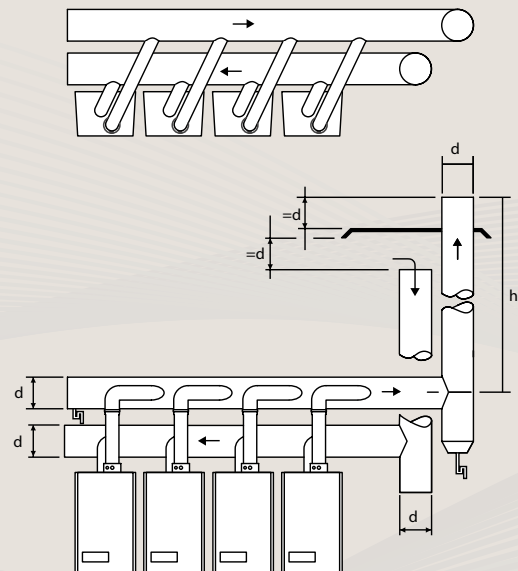
Room sealed system cascade
