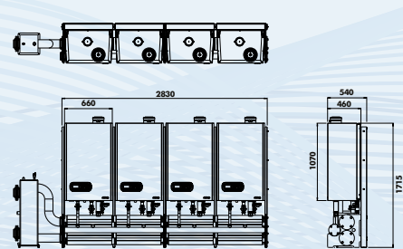
ATAG XL 4 boilers free standing in-line
