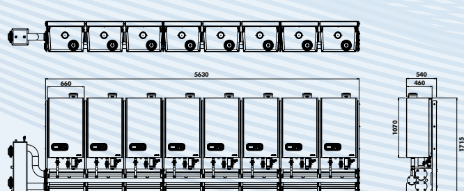
ATAG XL 8 boilers free standing in-line
