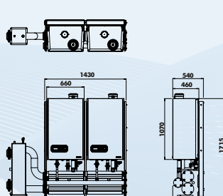
ATAG XL 2 boilers free standing in-line
