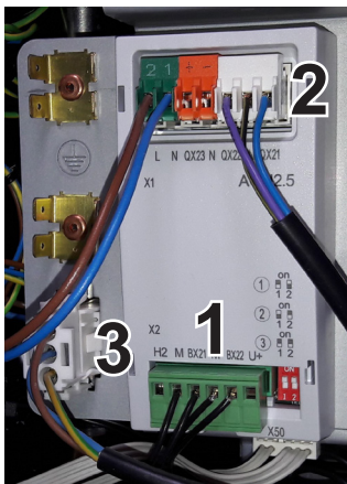
Clip-In-Modul
