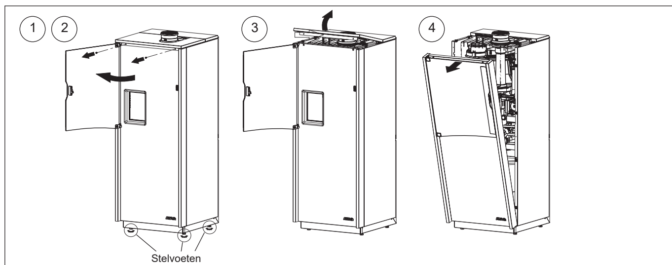
demontage manteldelen
