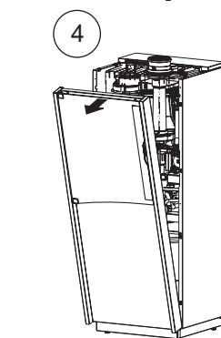
demontage manteldelen QR-CC
