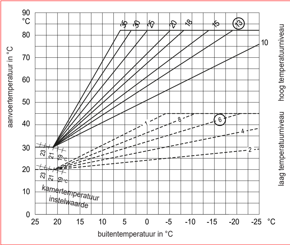
Stooklijn
