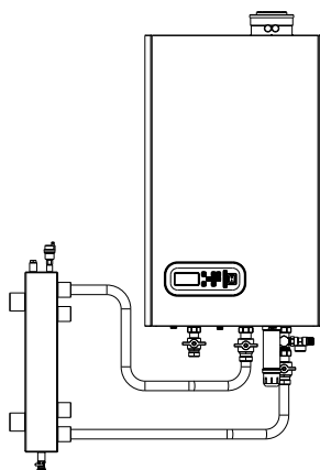
XL 1 ketel, wandhangend
