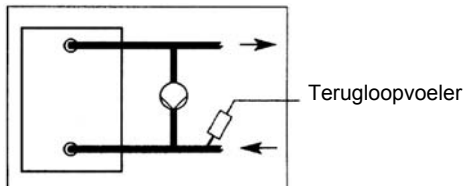
Bypassschakeling met terugloop- Bypasspomp
